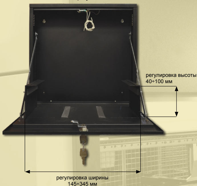
AWO529 – корпус DVR/SMALL/VERTICAL AWO529W – корпус DVR/SMALL/VERTICAL/WHITE
